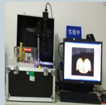
Portable cross section of terminal analyzer
